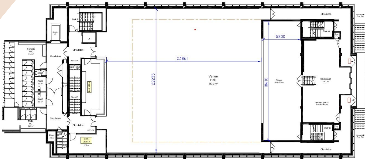
VENUE HALL PLAN @ 1:100
